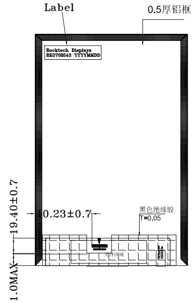
FPC折弯示意图 FPC Fold Shipment
